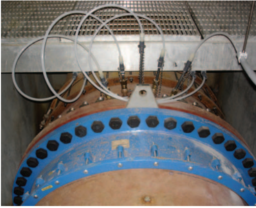
Westfall Model 2800 Static Mixer in-line at Sebago Lake Water Treatment Facility.
